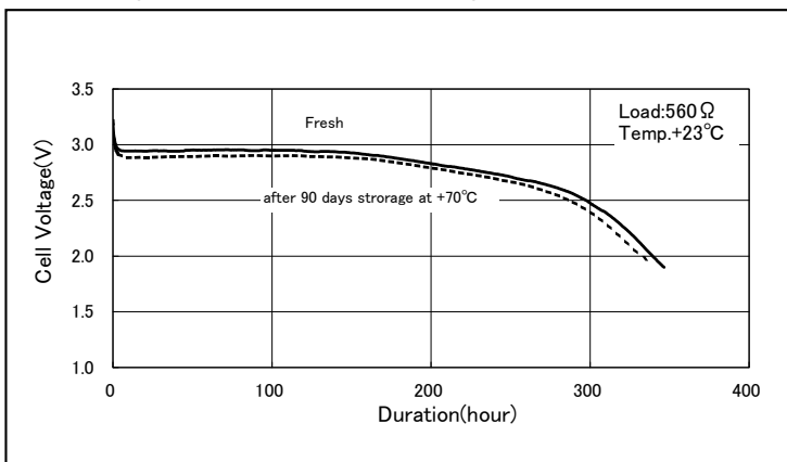
Discharge Characteristics after storage of CR17335E-N
