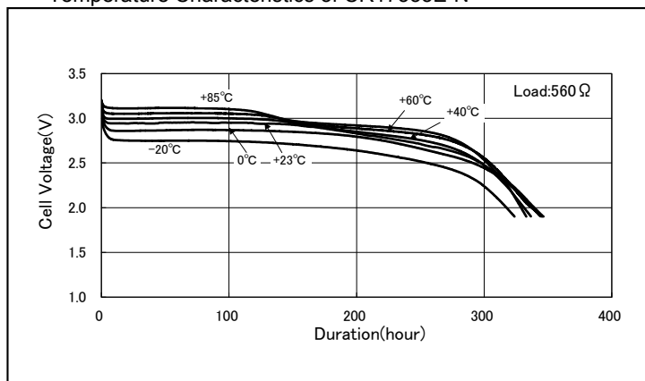
Temperature Characteristics of CR17335E-N
