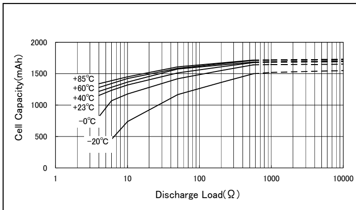
Discharge Load vs. Cell Capacity of CR17335E-N
