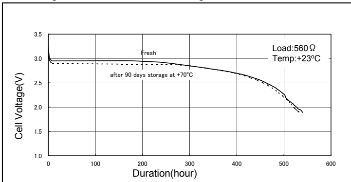
Discharge Characteristics after storage of CR17450E-N
