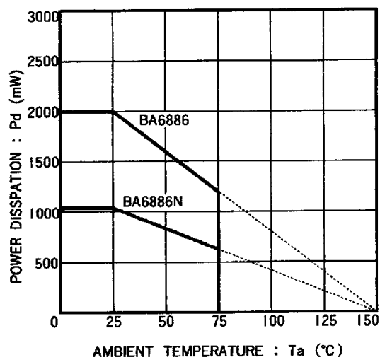
Figure 5 BA6886 and BA6886N
