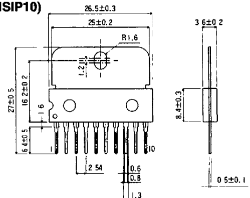
BA6886 (HSIP10)
