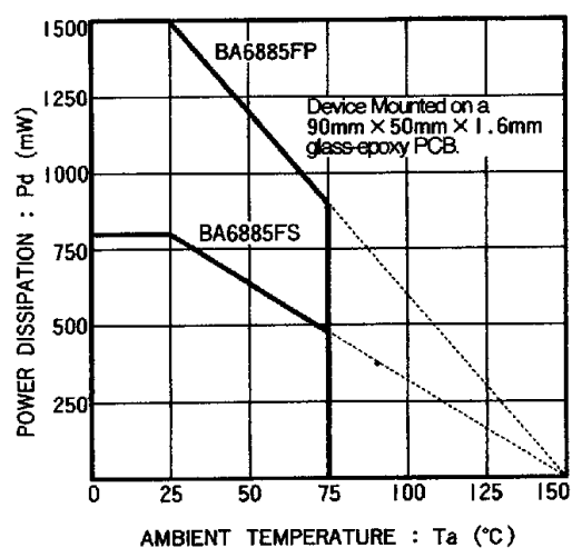
Figure 4 BA6885FS and BA6885FP
