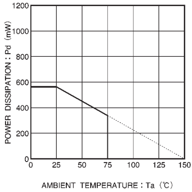
Fig.4 Power dissipation
