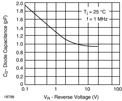
Figure 1. Diode Capacitance
