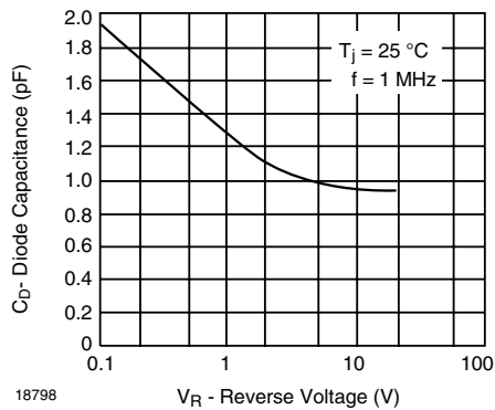
Figure 1. Diode Capacitance
