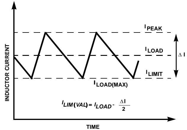
FIGURE 73. "VALLEY" CURRENT LIMIT THRESHOLD POINT
