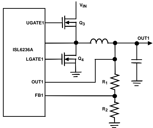
FIGURE 77. SETTING V_{OUT1} WITH A RESISTOR DIVIDER
