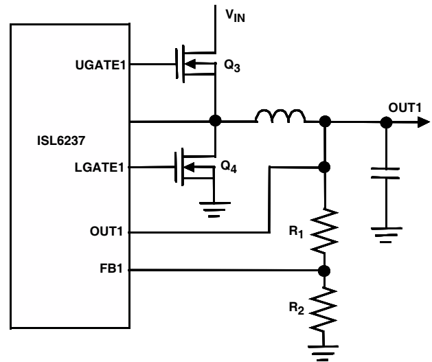
FIGURE 71. SETTING V_{OUT1} WITH A RESISTOR DIVIDER
