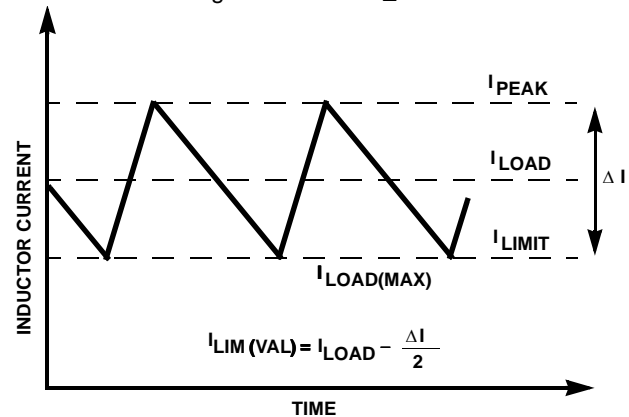
FIGURE 68. "VALLEY" CURRENT LIMIT THRESHOLD POINT
