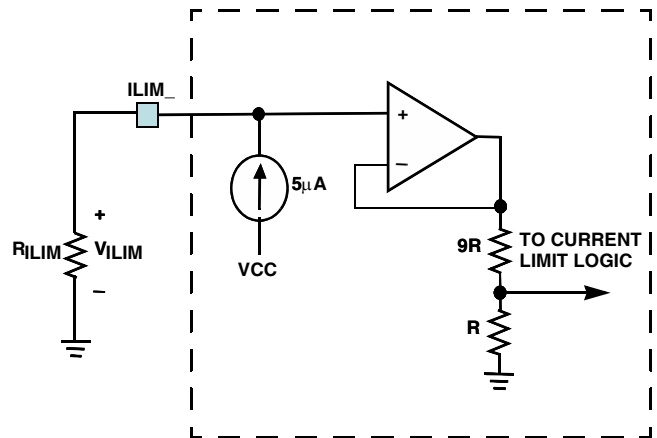
FIGURE 69. CURRENT LIMIT BLOCK DIAGRAM
