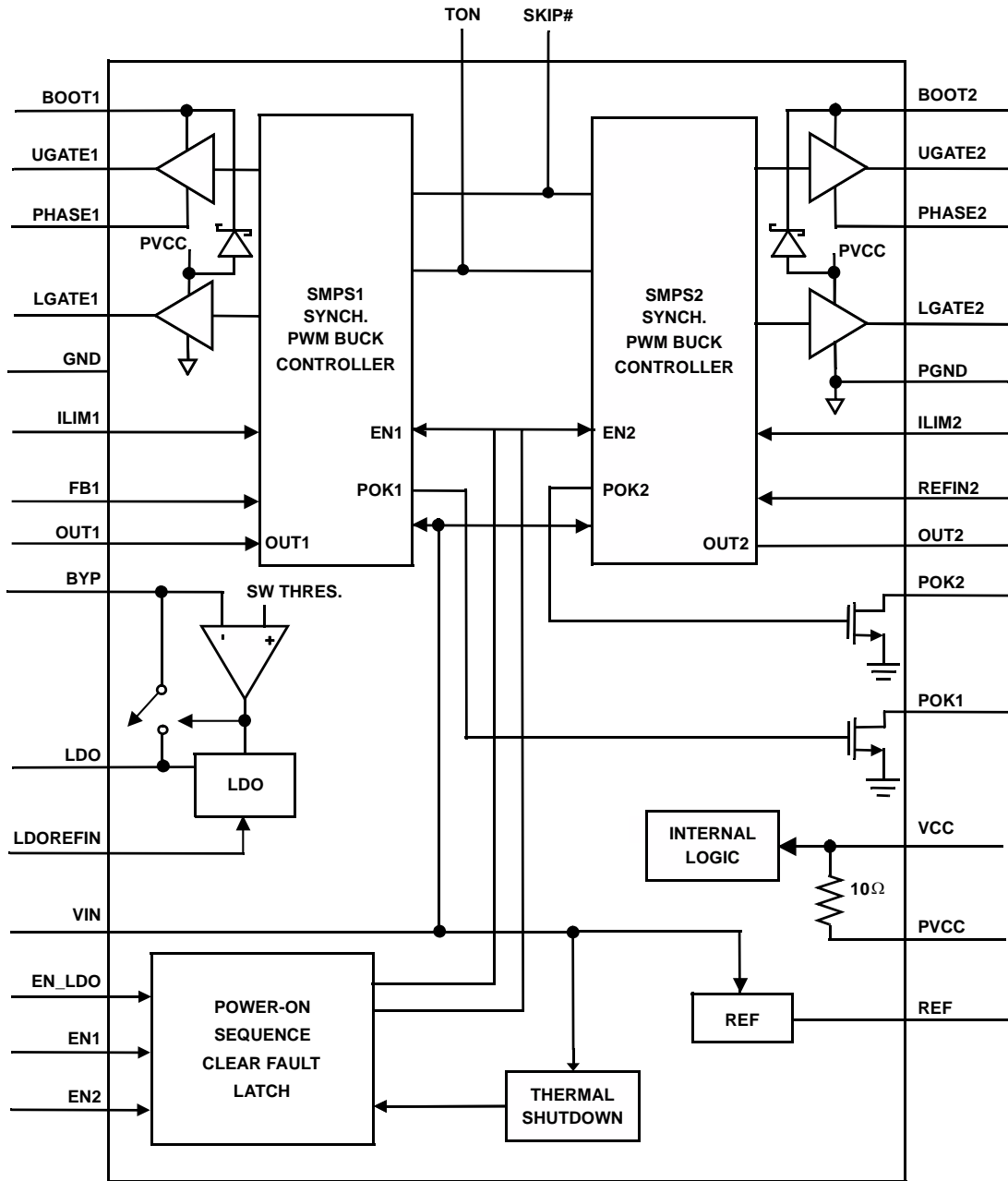
FIGURE 64. DETAIL FUNCTIONAL DIAGRAM ISL6237
