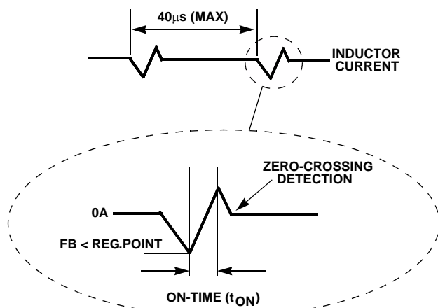
FIGURE 67. ULTRASONIC CURRENT WAVEFORMS
