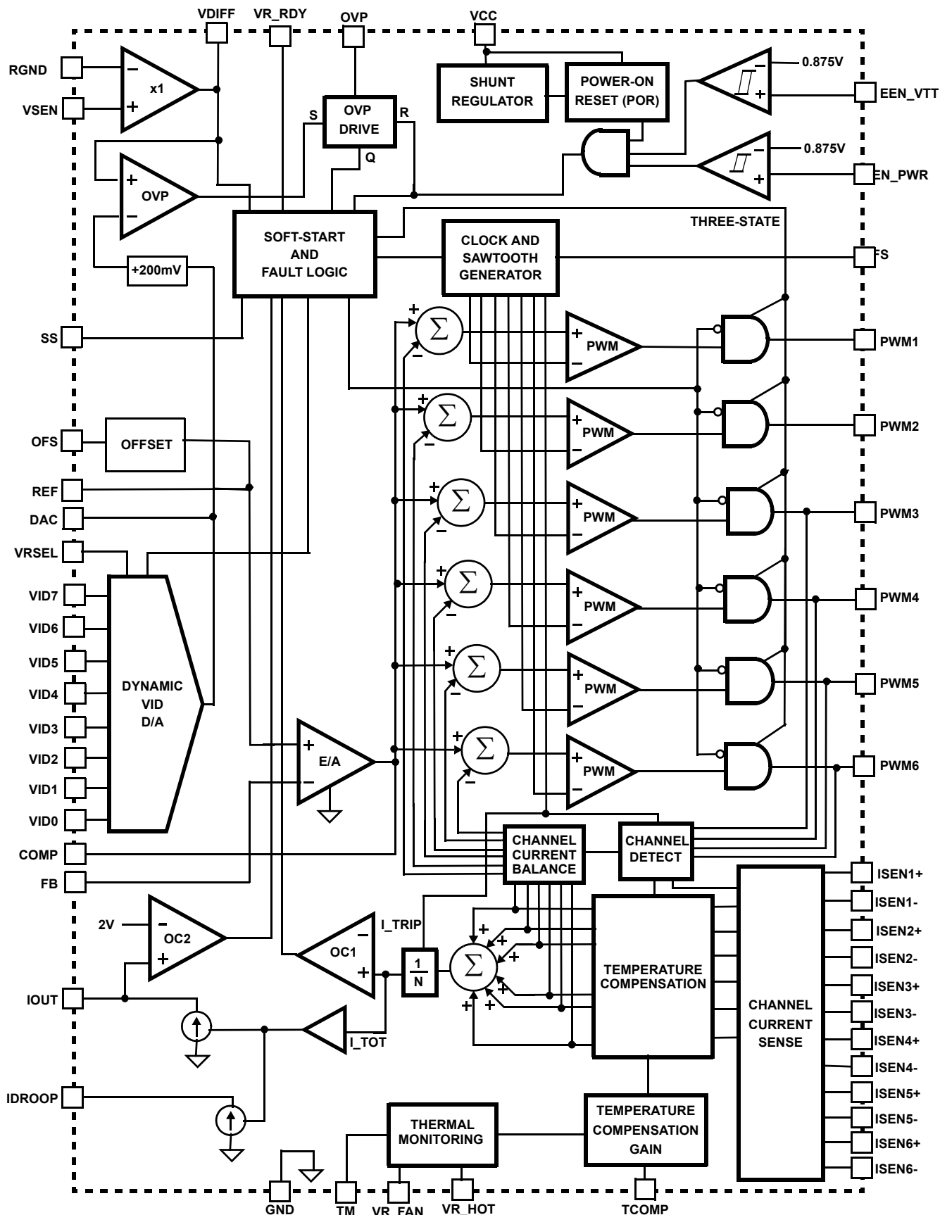
ISL6307B Block Diagram
