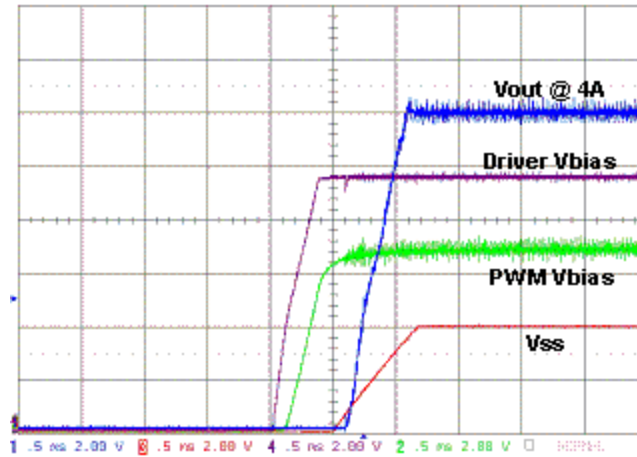
FIGURE 17. OUTPUT SOFT-START
