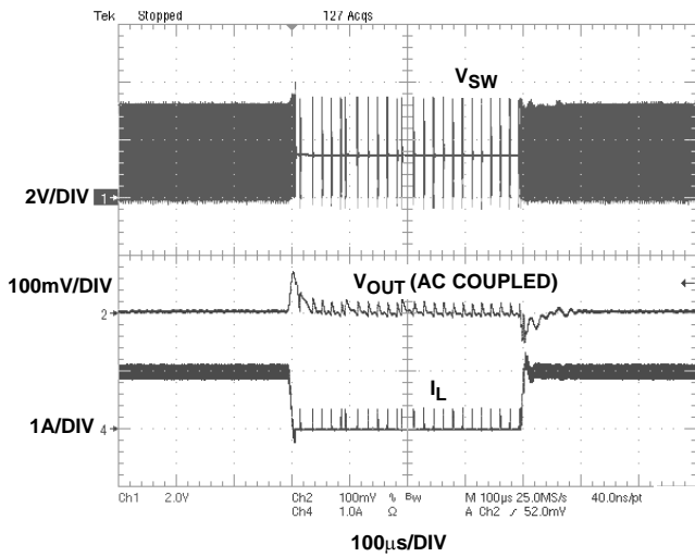
FIGURE 17. LOAD TRANSIENT TEST (MODE = V_{IN} = 3.6V ; V_O = 1.5V ; I_O = 0.01A\sim 1A )
