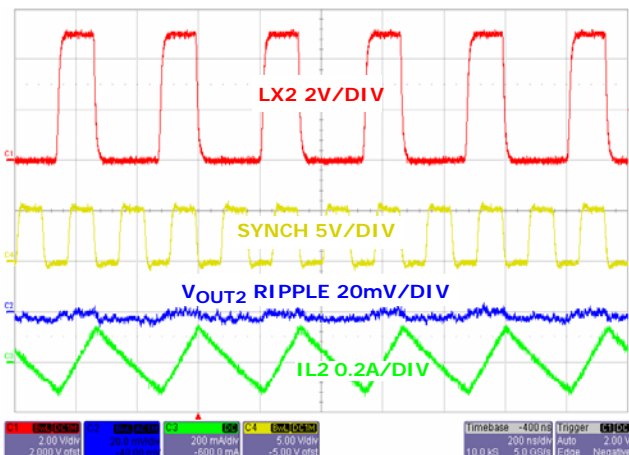
FIGURE 24. CHANNEL 2 STEADY STATE OPERATION AT NO LOAD WITH FREQUENCY = 6MHz
