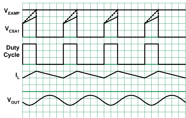
FIGURE 39. PWM OPERATION WAVEFORMS
