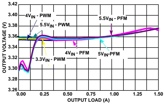
FIGURE 9. V_{OUT} REGULATION vs LOAD, V_{OUT} = 3.3\text{V}
