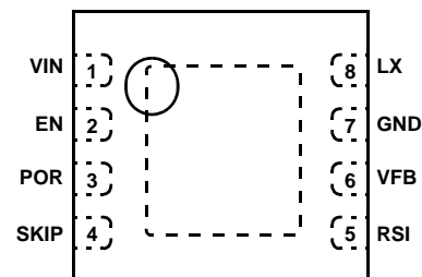
ISL8009A (8 LD DFN) TOP VIEW
