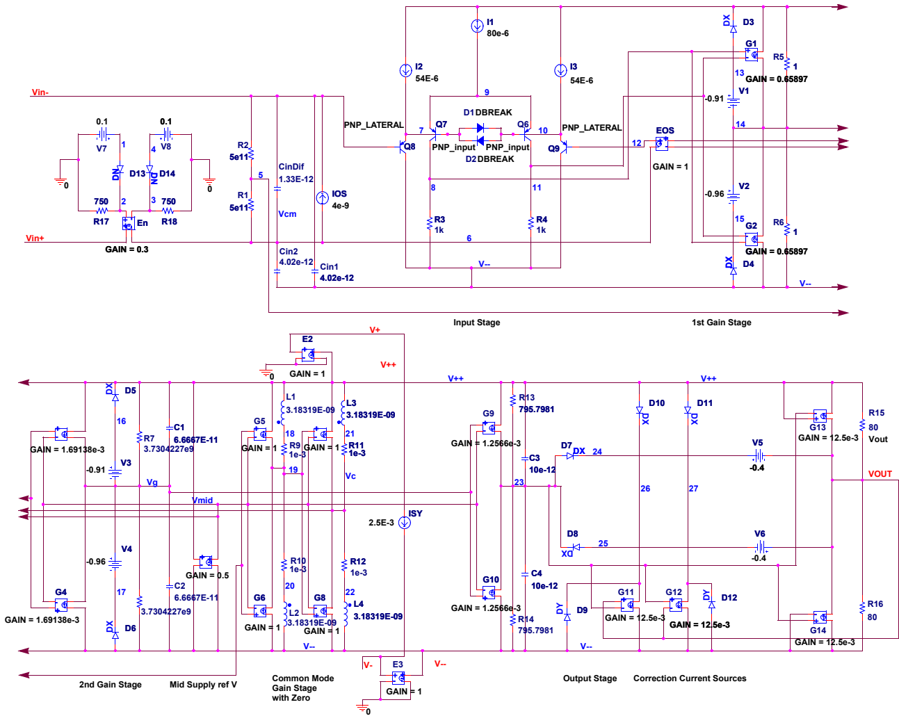
FIGURE 50. SPICE SCHEMATIC
