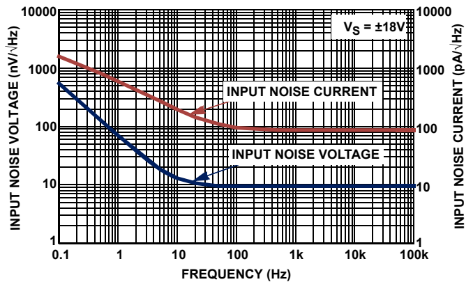
FIGURE 2. INPUT NOISE PERFORMANCE
