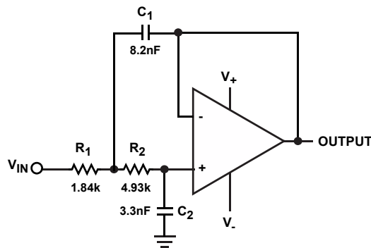
SALLEN-KEY LOW PASS FILTER (10kHz) FIGURE 1. TYPICAL APPLICATION
