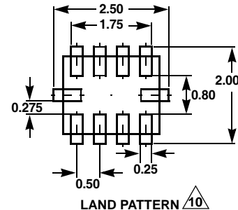
LAND PATTERN 10
