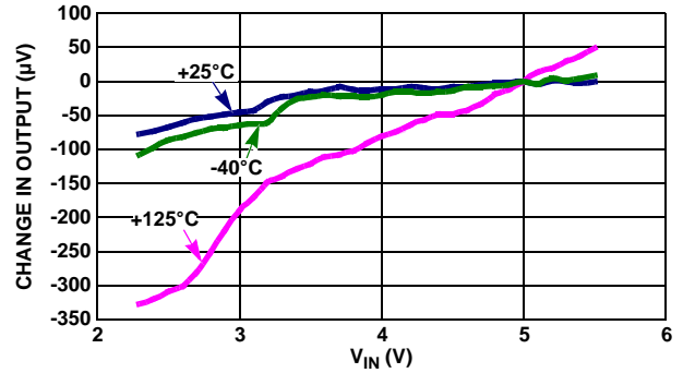
FIGURE 52. LINE REGULATION OVER-TEMPERATURE
