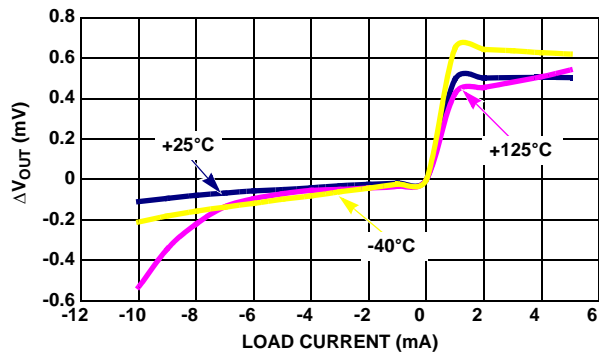
FIGURE 21. LOAD REGULATION
