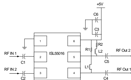
FIGURE 29. APPLICATION CIRCUIT
