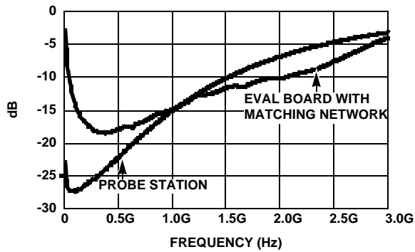
FIGURE 32. |S_{11}| vs FREQUENCY
