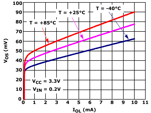
FIGURE 18. INPUT TO OUTPUT OFFSET VOLTAGE vs SINK CURRENT vs TEMPERATURE
