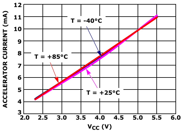
FIGURE 19. ACCELERATOR PULL-UP CURRENT vs V_{CC}
