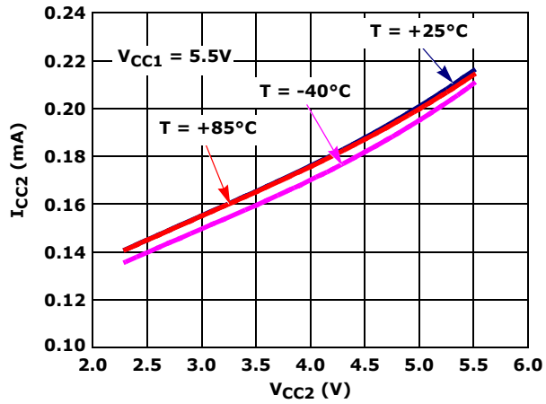
FIGURE 13. I_{CC2} ENABLED CURRENT vs V_{CC2} (ISL33002 AND ISL33003)
