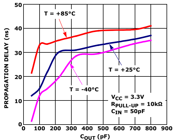
FIGURE 22. PROPAGATION DELAY H-L vs C_{OUT}
