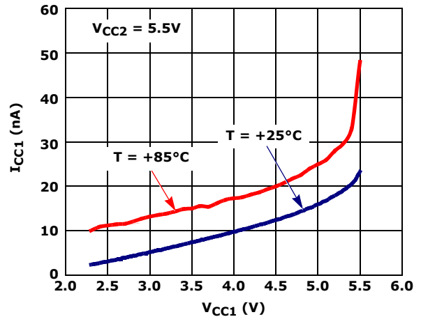
FIGURE 12. I_{CC1} DISABLED CURRENT vs V_{CC1} (ISL33003)
