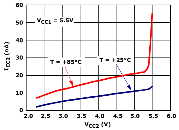
FIGURE 14. I_{CC2} DISABLED CURRENT vs V_{CC2} (ISL33003)
