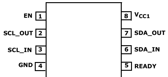
ISL33001 (8 LD MSOP) TOP VIEW
