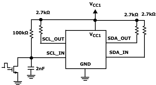
FIGURE 6. ACCELERATOR CURRENT TEST CIRCUIT
