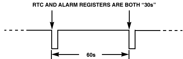
FIGURE 14. \overline{\text{IRQ}}/\text{F}_{\text{OUT}} WAVEFORM
