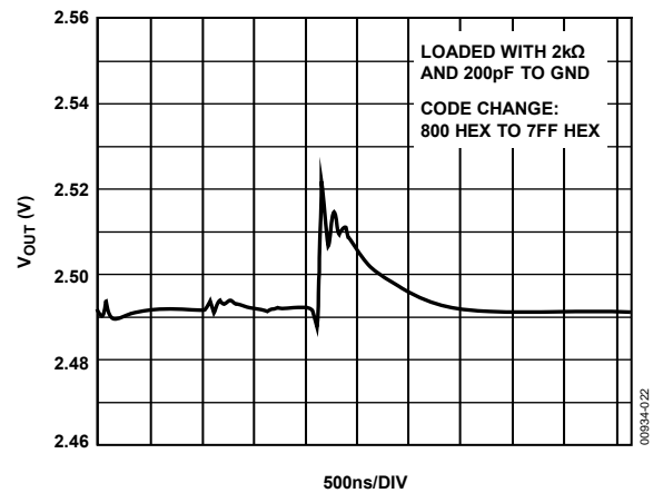
500ns/DIV
