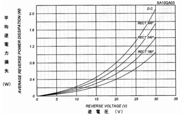
FIG.4 平均逆電力損失 AVERAGE REVERSE POWER DISSIPATION
