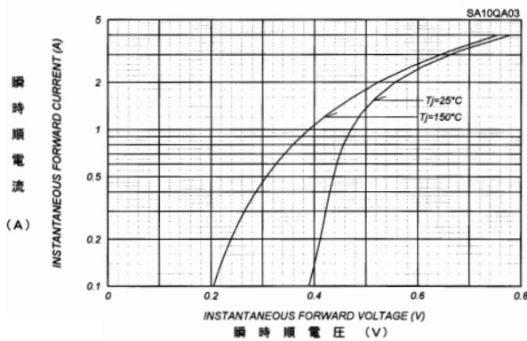
FIG.1 順電圧特性 FORWARD CURRENT VS. VOLTAGE
