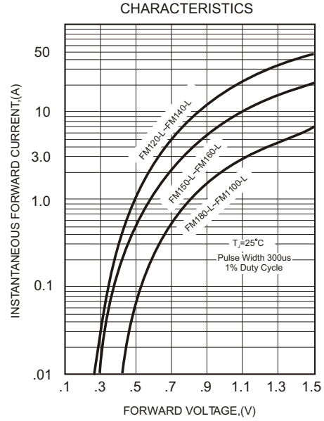
FIG.2-TYPICAL FORWARD CHARACTERISTICS
