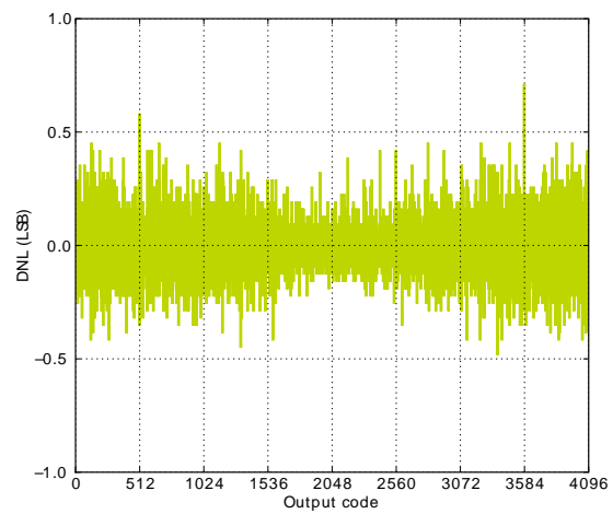
5VDIFF Reference
