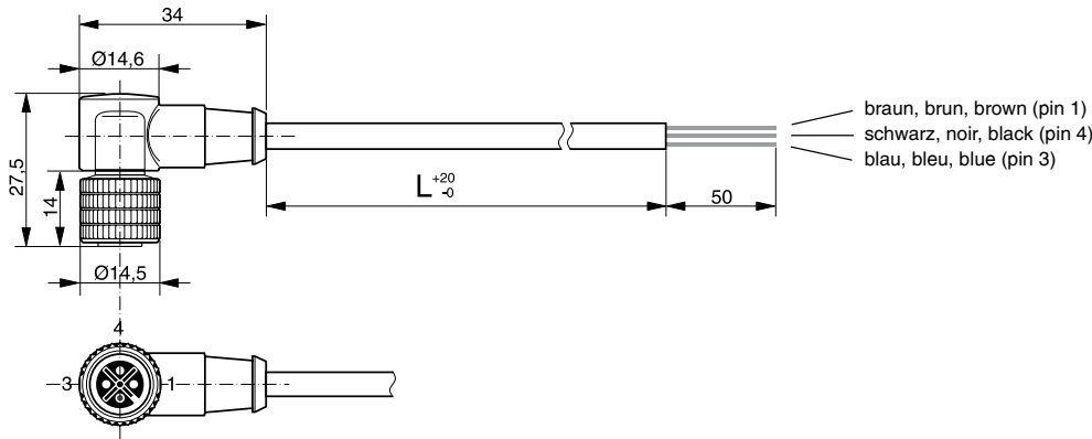
Winkel / coudé / right angle
