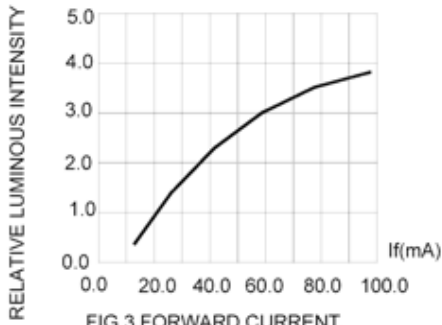
FIG.3 FORWARD CURRENT.
