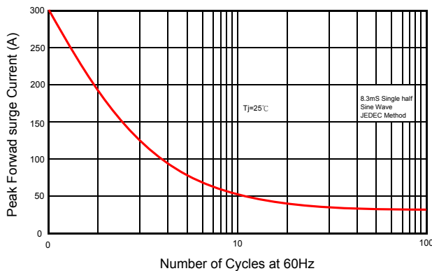
Maximum Non- Repetitive Forward Surge Current
