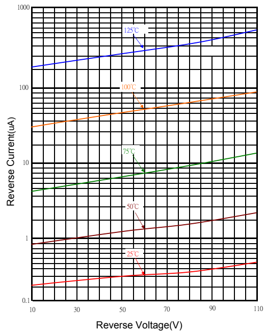
Typical Reverse Characteristic
