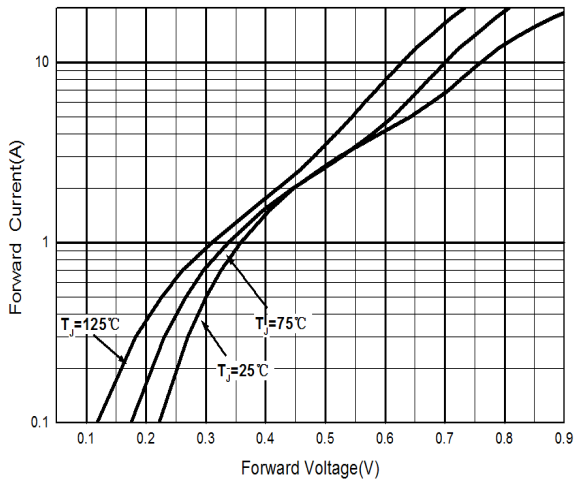
Figure 1: Typical Forward Characteristics Figure 2: Typical Capacitance Characteristics
