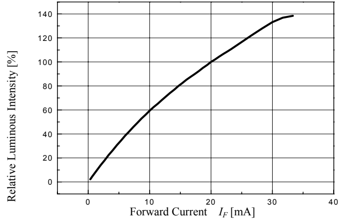
Intensity vs Forward Current ( T_A=25^\circ\text{C} )
