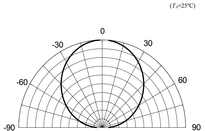
Radiation Diagram
