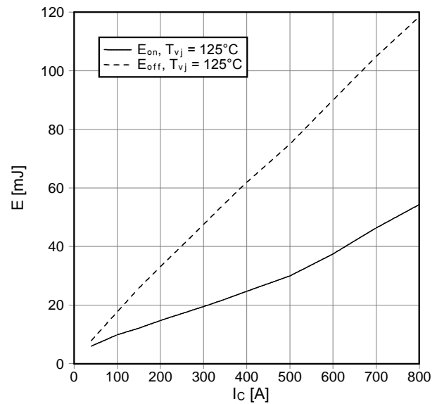
Schaltverluste IGBT-Wechselr. (typisch) switching losses IGBT-inverter (typical) E_{on} = f(I_c) , E_{off} = f(I_c) V_{GE} = \pm 15\text{ V} , R_{Gon} = 1,8\ \Omega , R_{Goff} = 1,8\ \Omega , V_{CE} = 600\text{ V}
