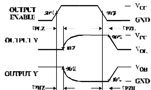
Figure 2. Switching Waveforms
