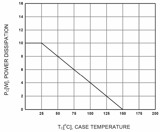
Figure 8. Power Derating
