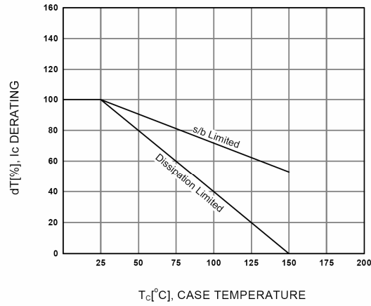
Figure 7. Derating Curve of Safe Operating Areas
