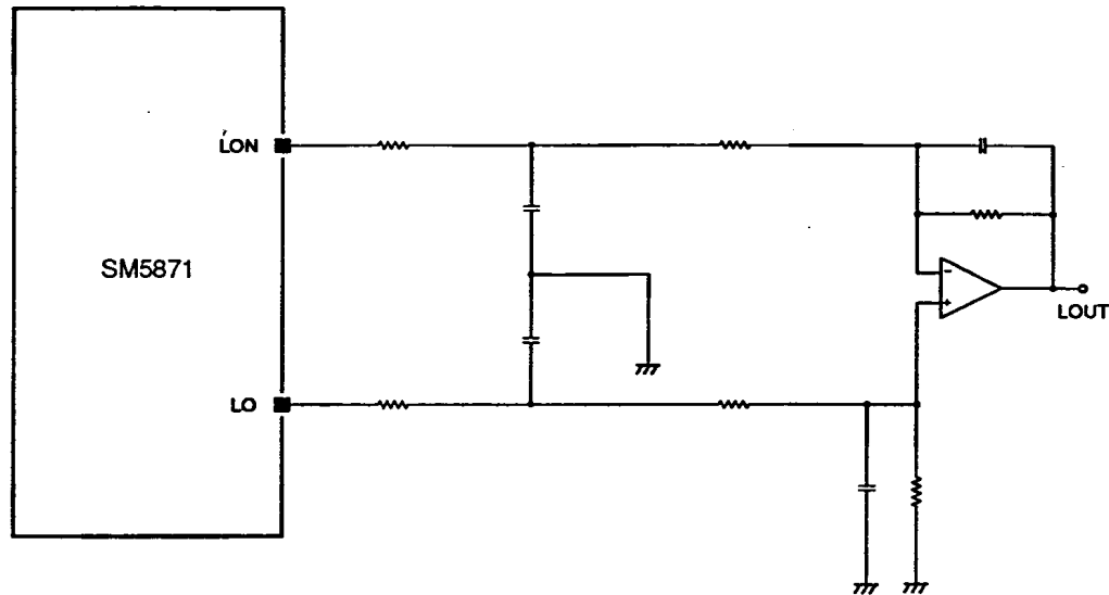
Figure 19. Output interface 2
