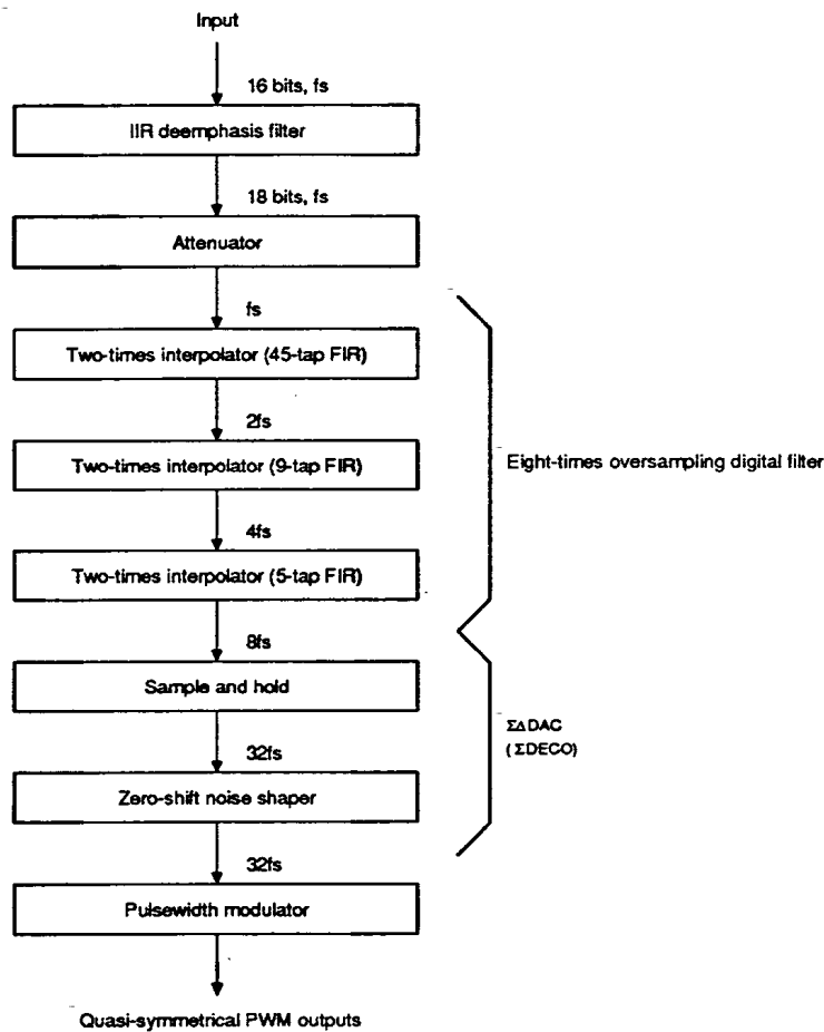
Figure 1. Arithmetic operation
