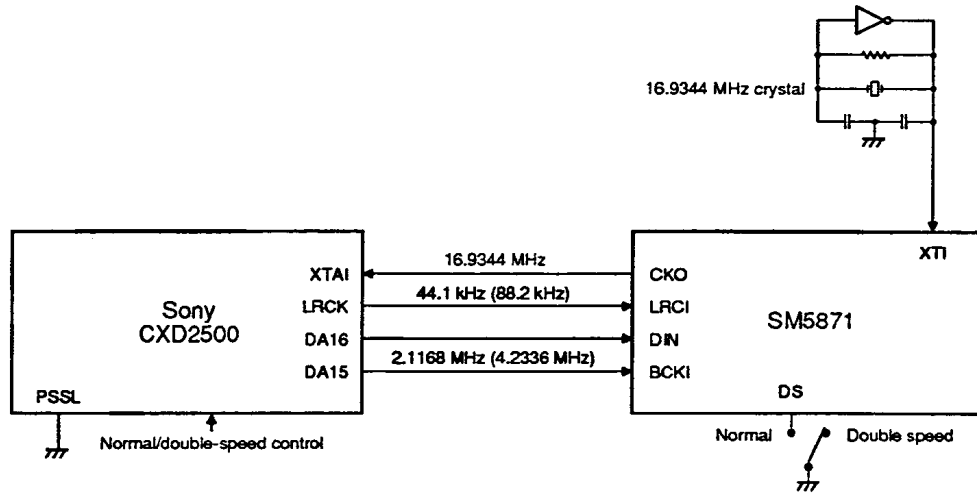
Figure 17. Sony CXD2500 interface
