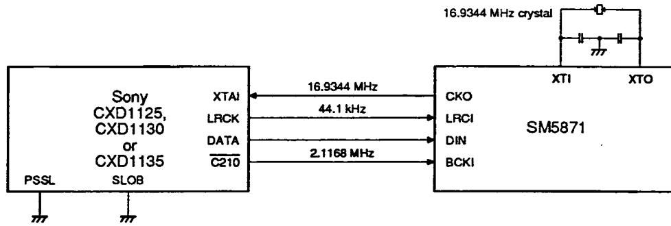
Figure 13. Sony CXD1125, CXD1130, CXD1135 interface
