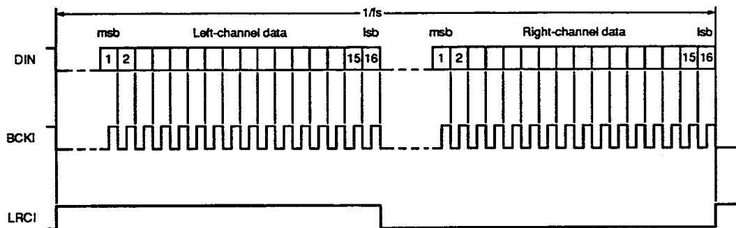
Figure 10. Audio data format 2
