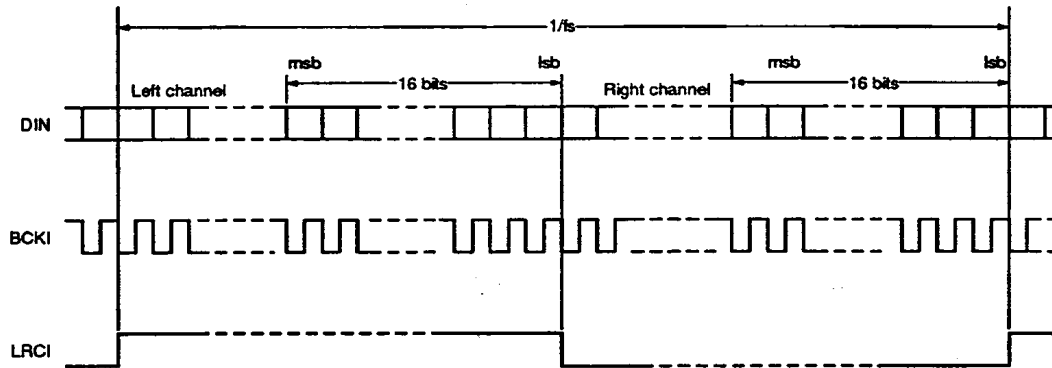
Figure 9. Audio data format 1
