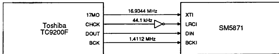
Figure 16. Toshiba TC9200F interface
