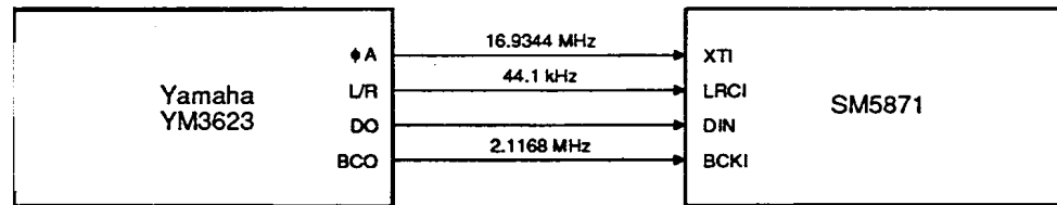
Figure 15. Yamaha YM3623 interface
