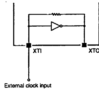
Figure 6. External system clock connection
