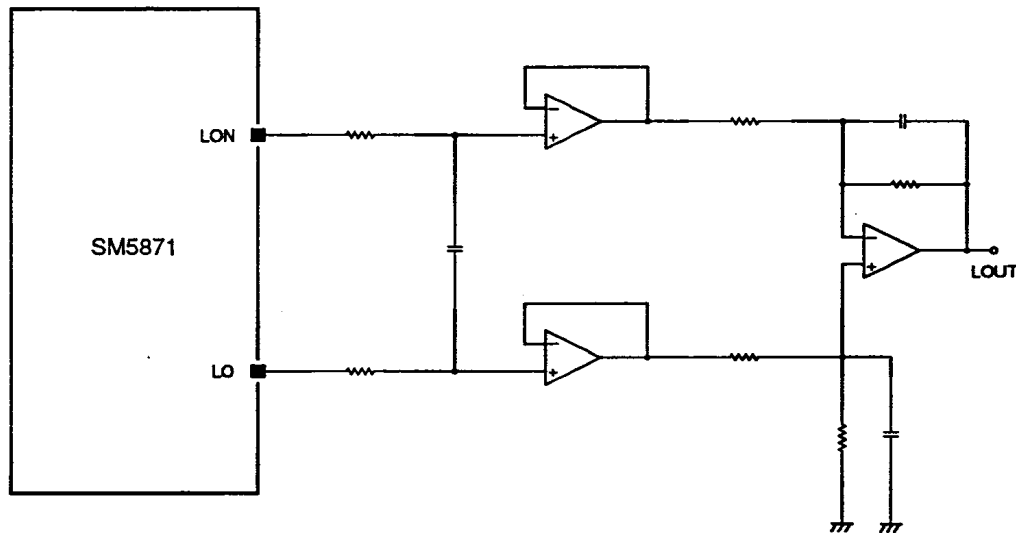
Figure 18. Output interface 1
