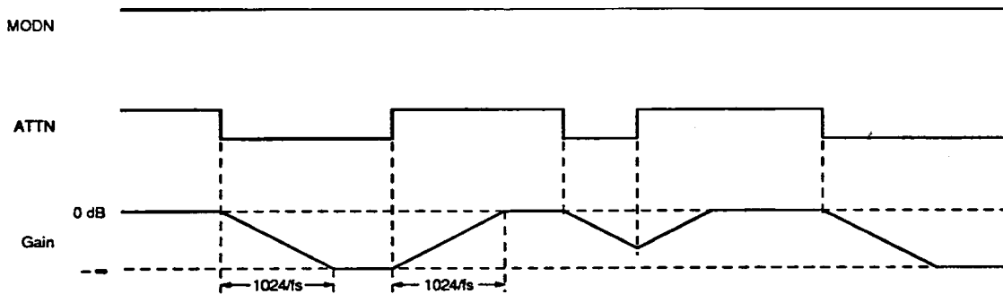
Figure 2. Fade in/out control
