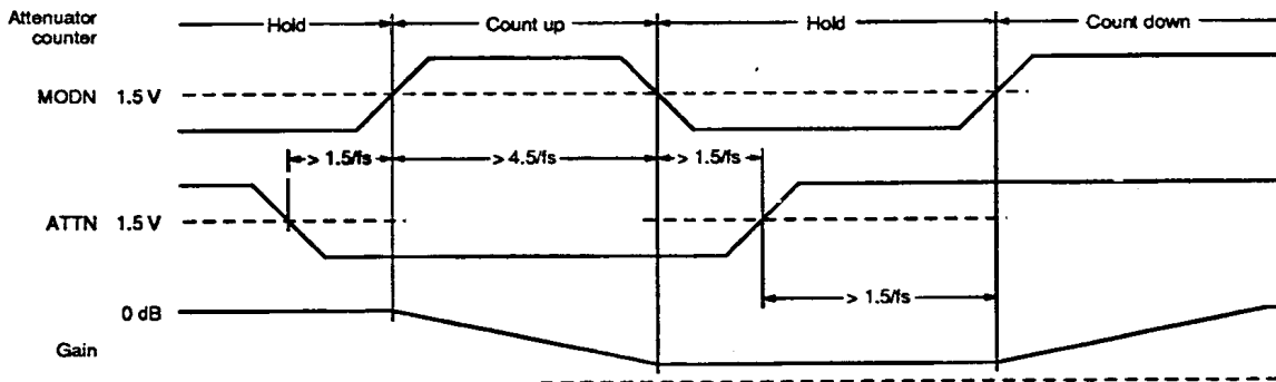
Figure 3. ATTN and MODN timing
