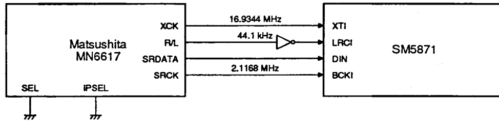
Figure 14. Matsushita MN6617 interface
