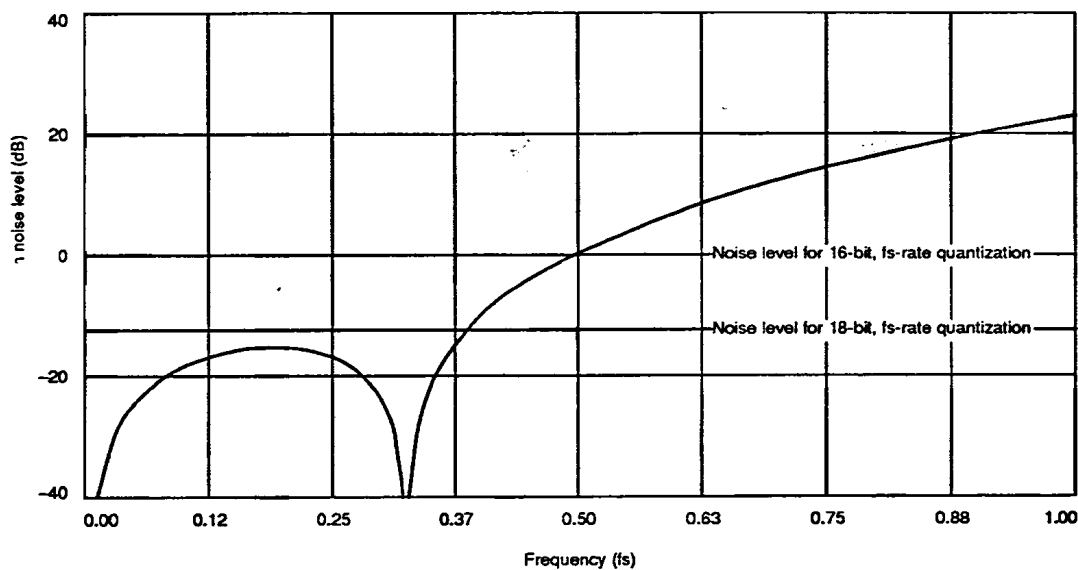
Figure 7. Requantizer noise characteristic
