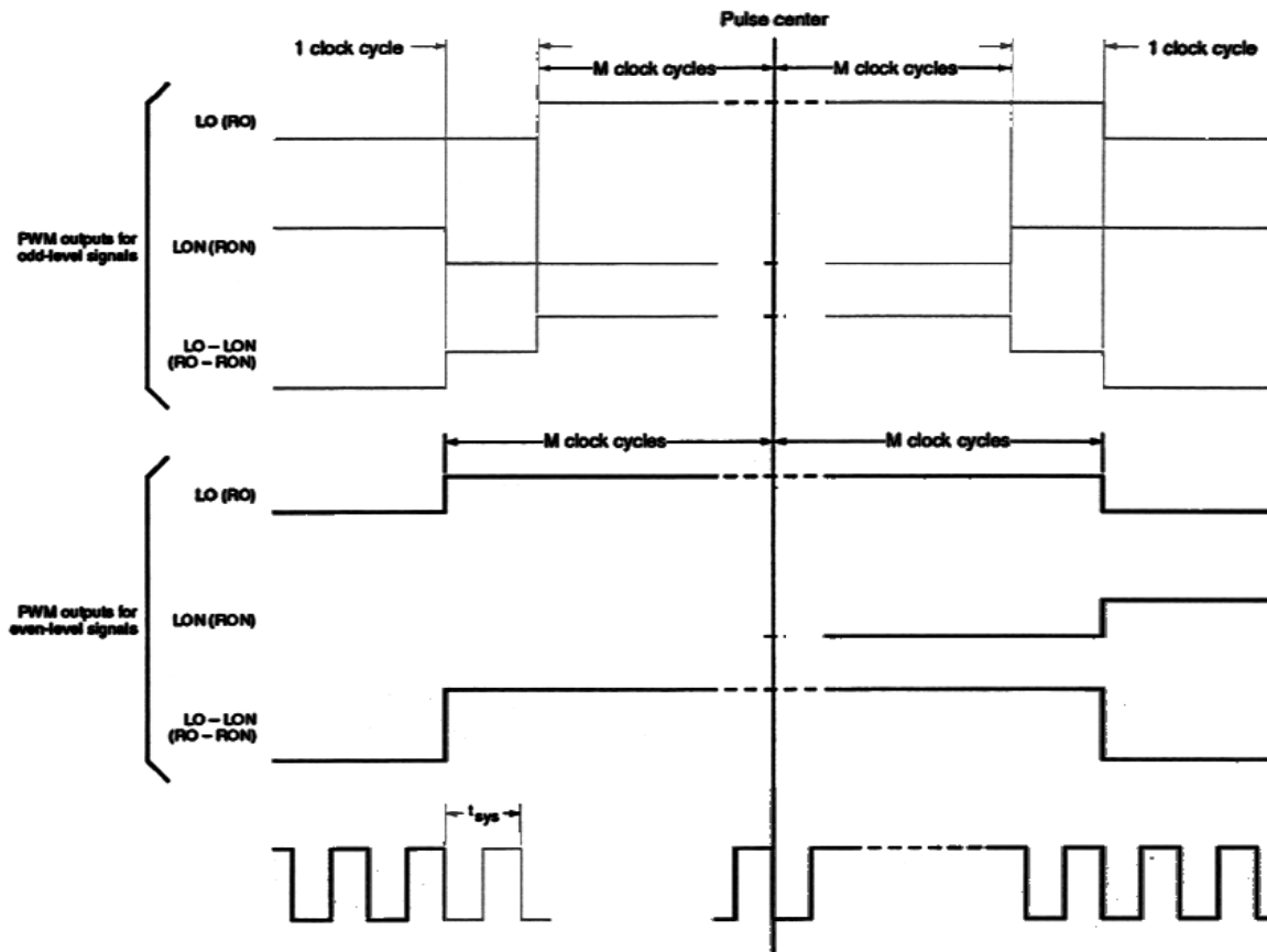
Figure 8. Pulsewidth modulation waveforms
