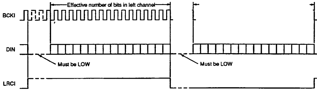
Figure 11. Mute detect timing
