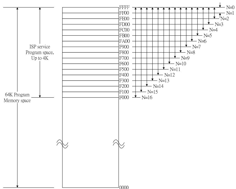
Fig. 3-1: SM59R16G6 programmable Flash
