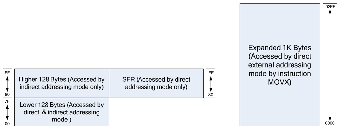
Fig. 3-3: RAM architecture
