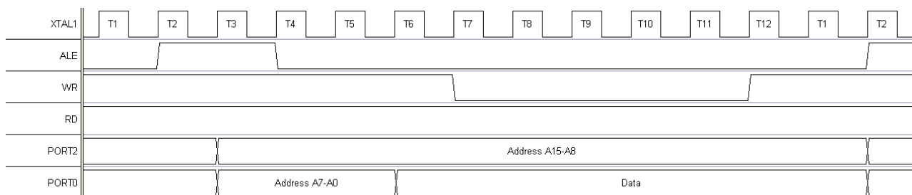
Fig 3-2 (b) : External memory access as write
