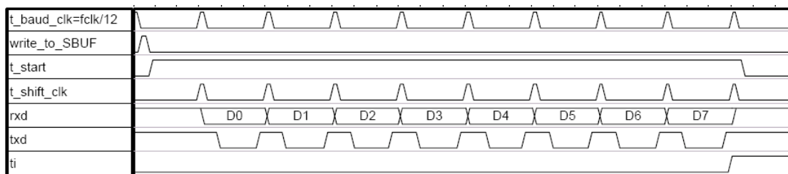
Fig. 8-1: Transmit mode 0 for Serial 0
