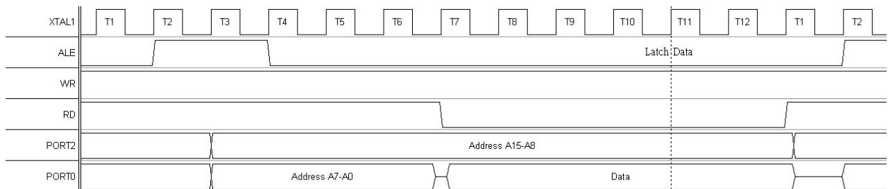
Fig 3-2 (a) : External memory access as read
