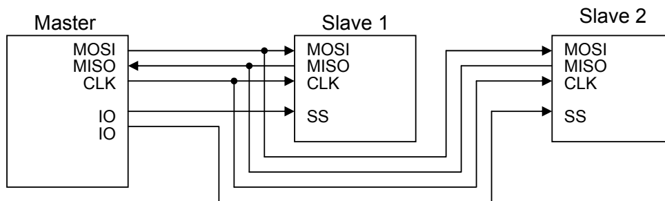
Fig. 14-1: SPI signals between master and slave devices
