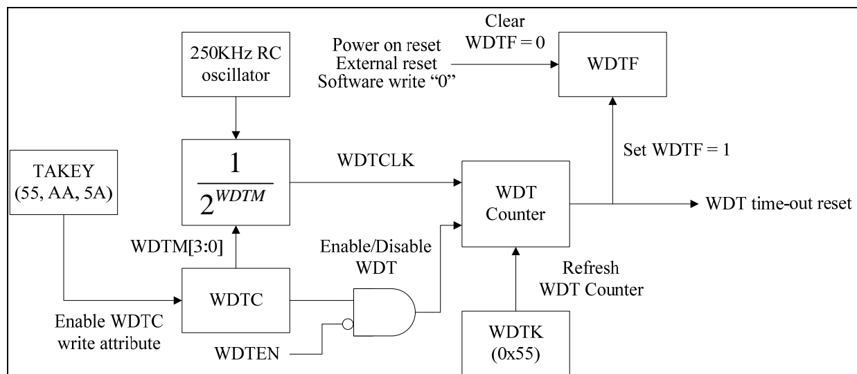
Fig. 9-1: Watchdog timer block diagram
