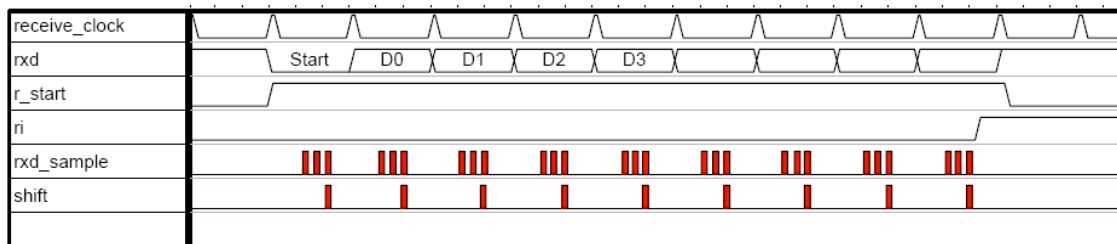
Fig. 8-4: Receive mode 1 for Serial 0
