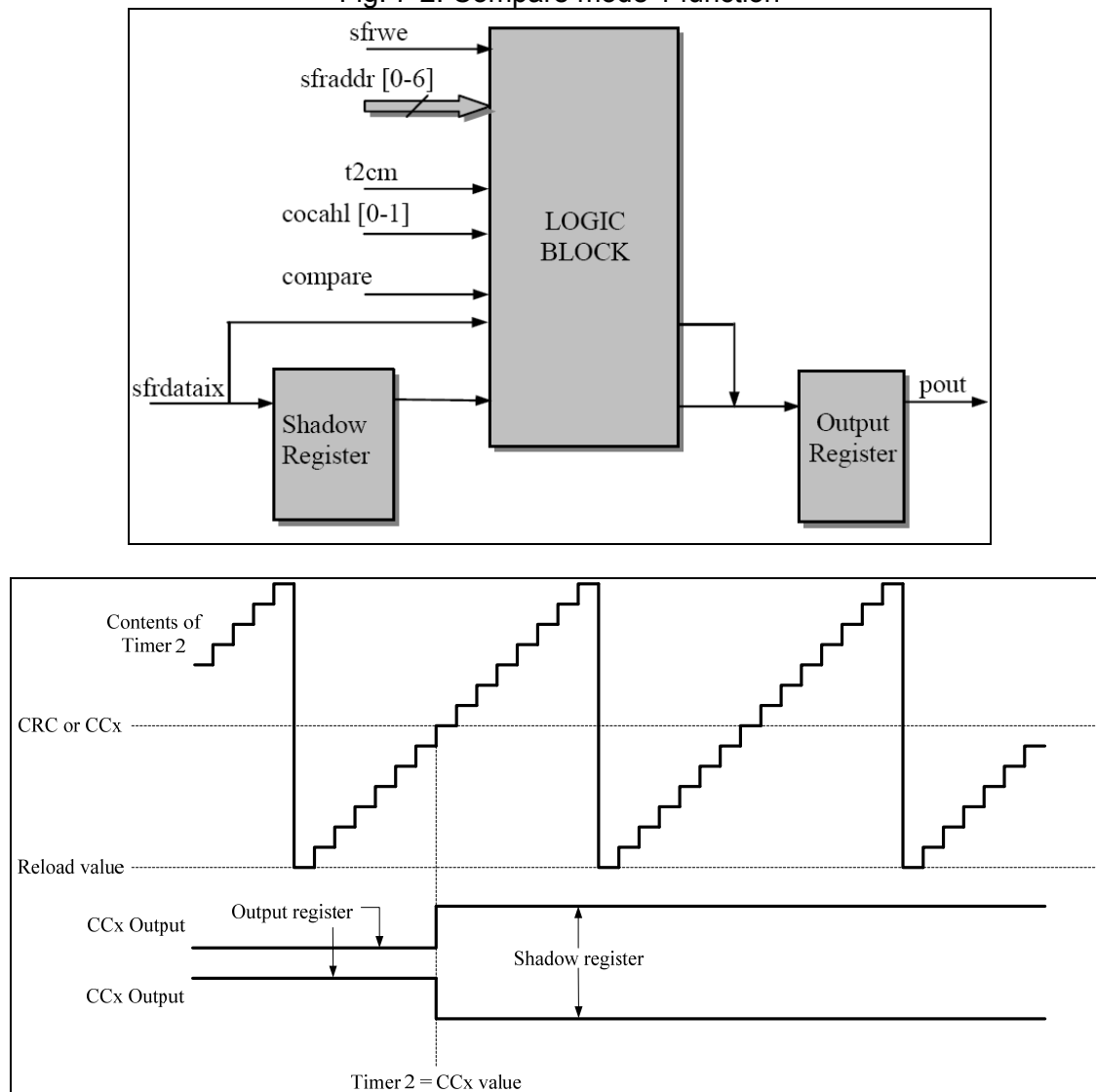
Fig. 7-2: Compare mode 1 function
