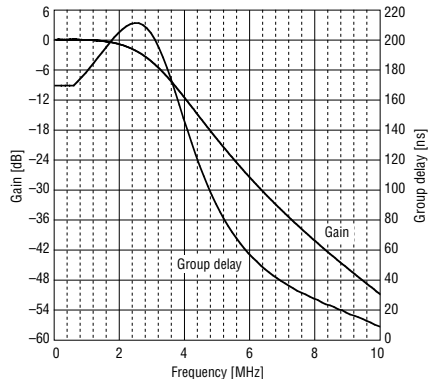
Figure 9. Gain and Group delay characteristics (half fc mode, FCDATA = 10)
