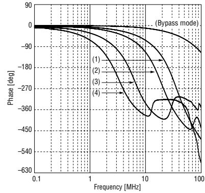
Figure 15. Phase vs. FCDATA, fc mode
