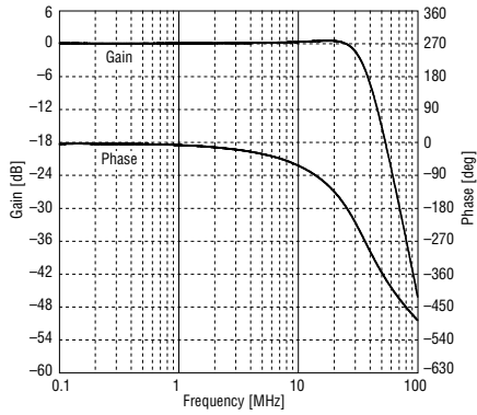
Figure 10. Gain and Phase characteristics (standard fc mode, FC DATA = 227)
