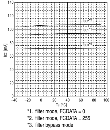
Figure 18. I_{CC1, 2, 3} vs. T_a
