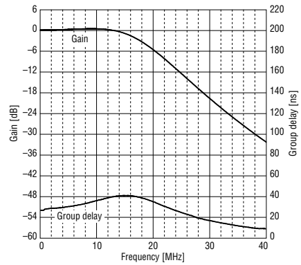
Figure 13. Gain and Group delay characteristics (half fc mode, FC DATA = 227)
