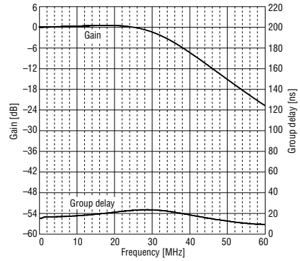
Figure 11. Gain and Group delay characteristics (standard fc mode, FC DATA = 227)
