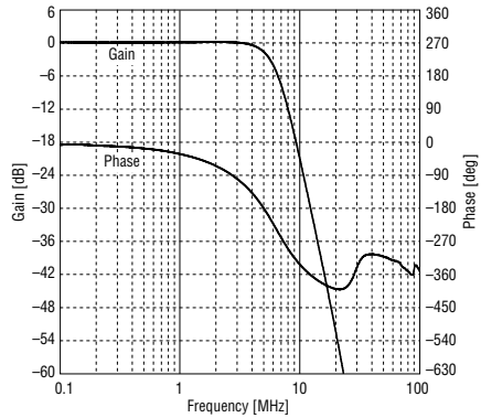
Figure 6. Gain and Phase characteristics (standard fc mode, FCDATA = 10)
