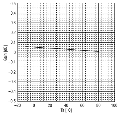
Figure 22. Gain vs. T_a
