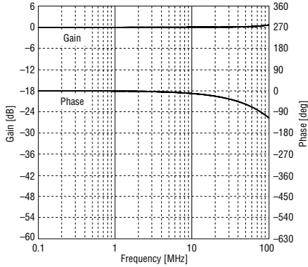
Figure 4. Gain and Phase characteristics (filter bypass mode)
