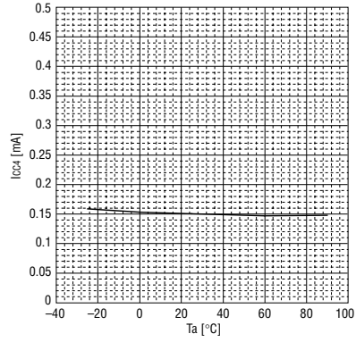
Figure 20. I_{CC4} vs. T_a
