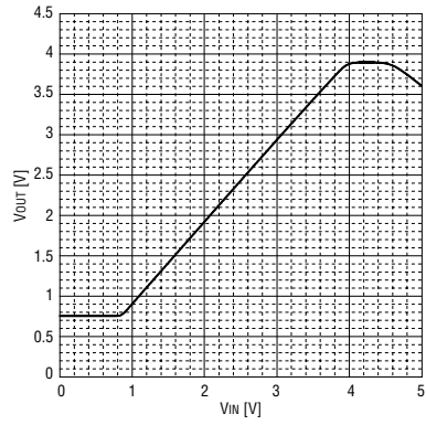
Figure 23. V_{IN} vs. V_{OUT} (filter mode, direct mode)
