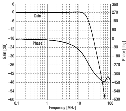
Figure 12. Gain and Phase characteristics (half fc mode, FC DATA = 227)
