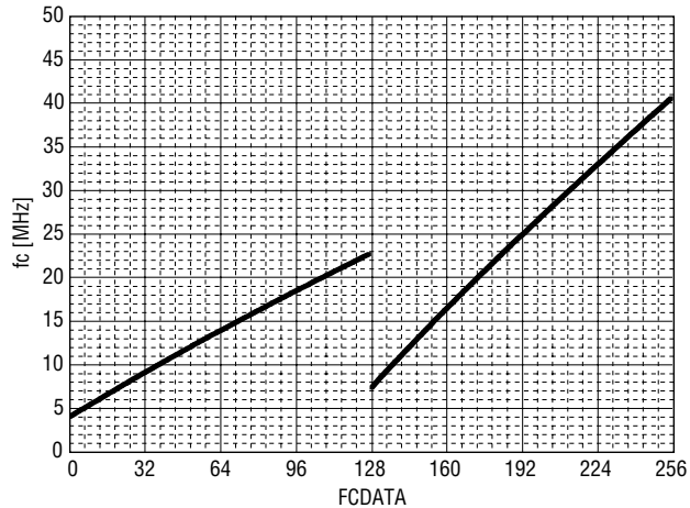
Figure 1. Cutoff frequency vs. FCDATA ( R_{ISET} = 1.8k\Omega )
