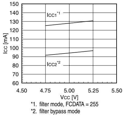
Figure 19. I CC1,2 vs. V CC (6dB, FCDATA = 255)
