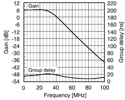
Figure 13. Gain and Group delay characteristics (6dB, standard fc mode, FC DATA = 227)
