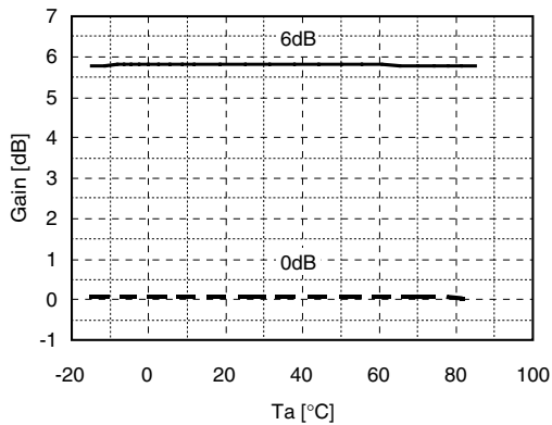
Figure 5. Gain vs. T_a
