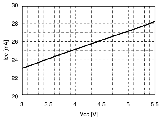
Figure 4. I_{CC} vs. V_{CC} (no signal input)
