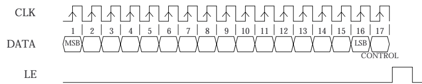
Figure 5. Serial data input
