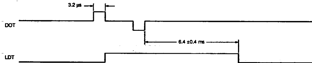
Figure 1. Lock detector timing
