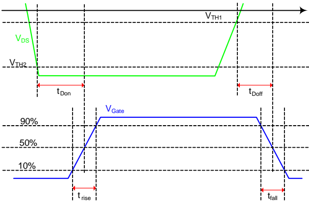
Timing waveform
