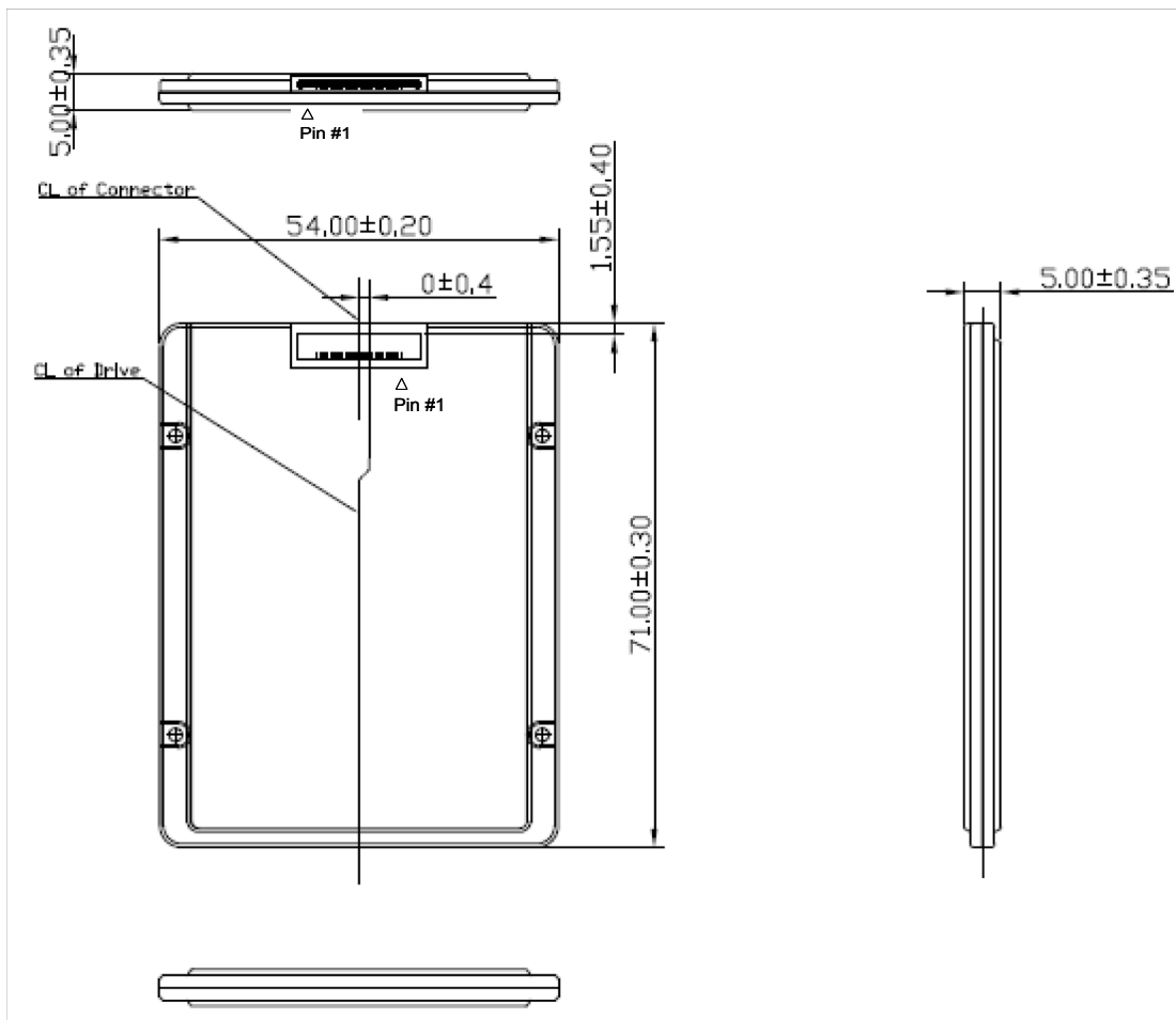
Figure 2-1. Physical dimension
