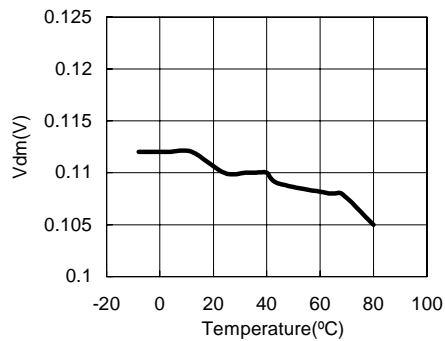
Differential Mode Bias Vdm vs. Temperature@Vtpwr=5V
