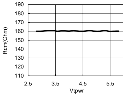
Common Mode Termination Resistance Rcm vs. Vtpwr at Temperature=24°C
