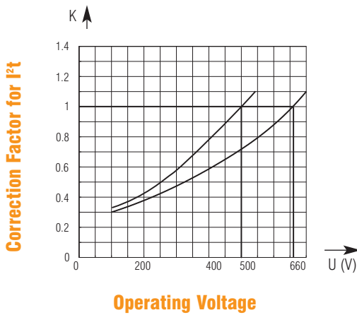
Correction factor to determine I 2 t value for a fuse operating below its rated voltage.
