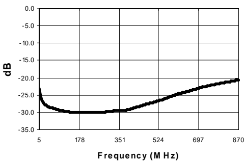
Return Loss: Coupling
