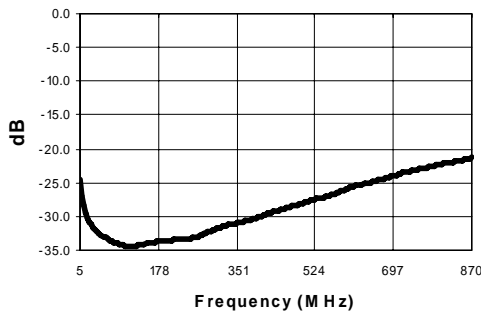
Return Loss: Output
