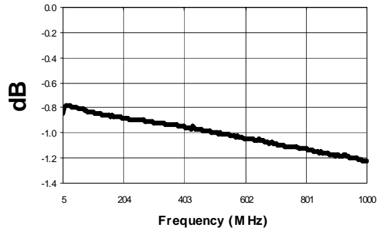
Mainline Loss
