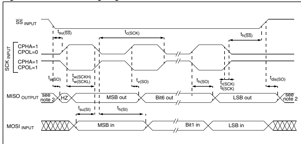
Figure 82. SPI slave timing diagram with CPHA = 1 (1)
