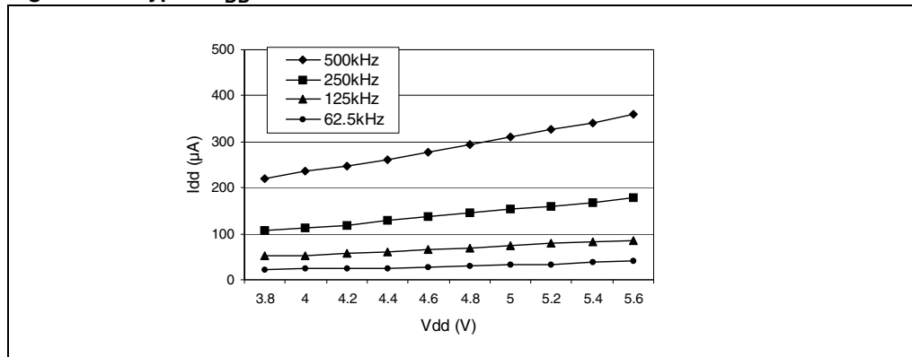
Figure 61. Typical I_{DD} in Slow mode
