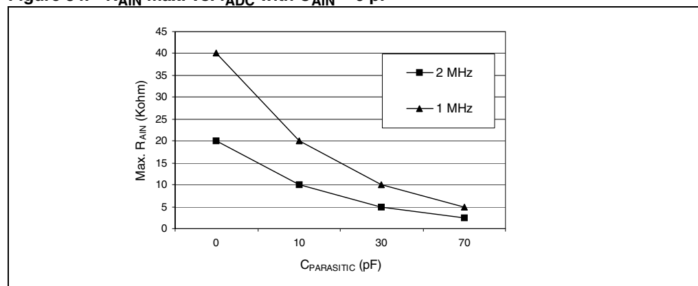
Figure 84. R_{AIN} max. vs. f_{ADC} with C_{AIN} = 0 pF (1)
