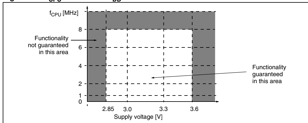
Figure 55. f_{\text{CPU max}} versus V_{\text{DD}}
