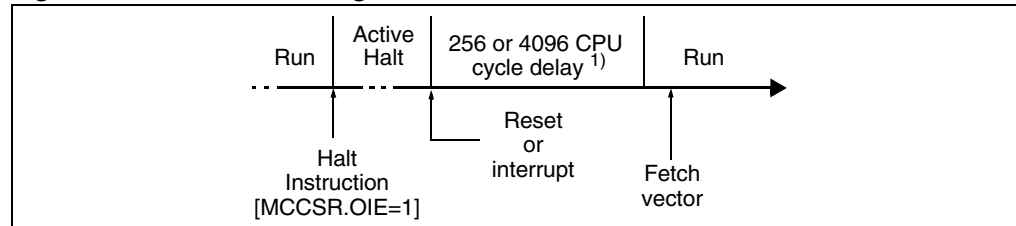
Figure 21. Active-Halt timing overview
