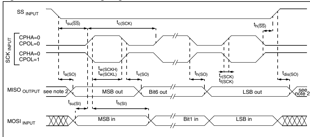
Figure 81. SPI slave timing diagram with CPHA = 0 (1)
