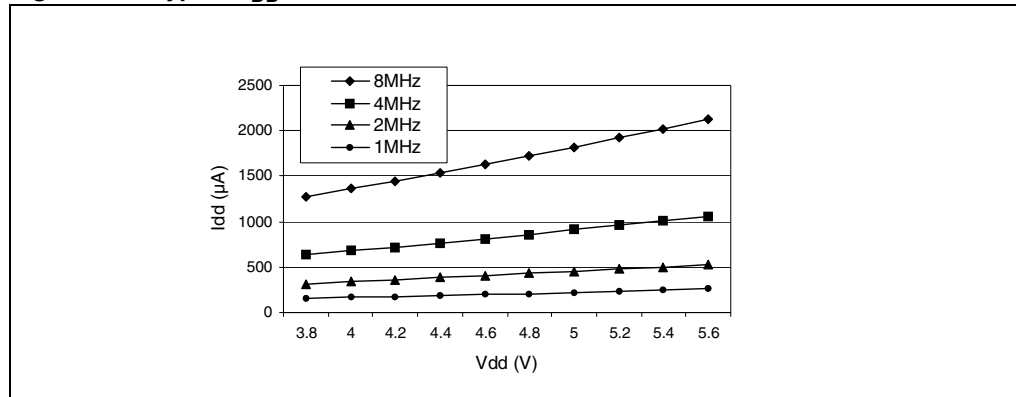
Figure 63. Typ. I_{DD} in Slow-Wait mode
