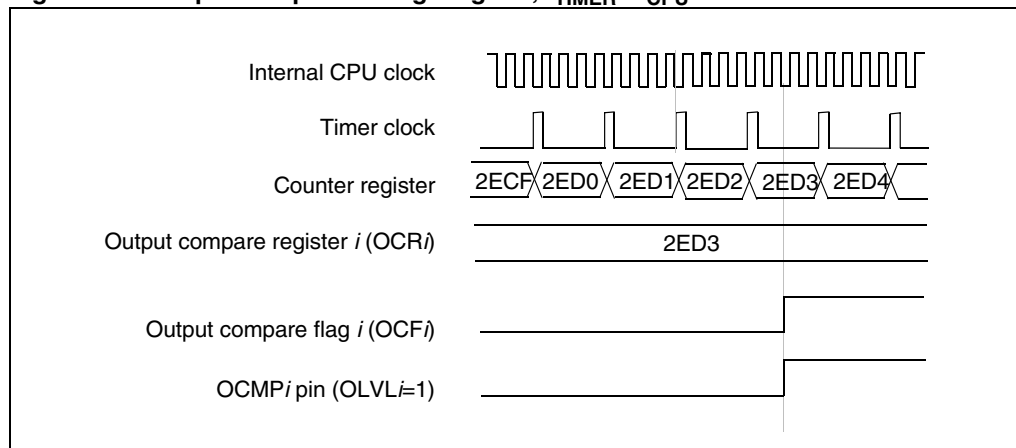
Figure 39. Output compare timing diagram, f_{TIMER} = f_{CPU}/4
