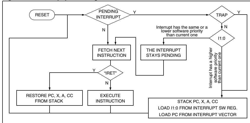
Figure 13. Interrupt processing flowchart
