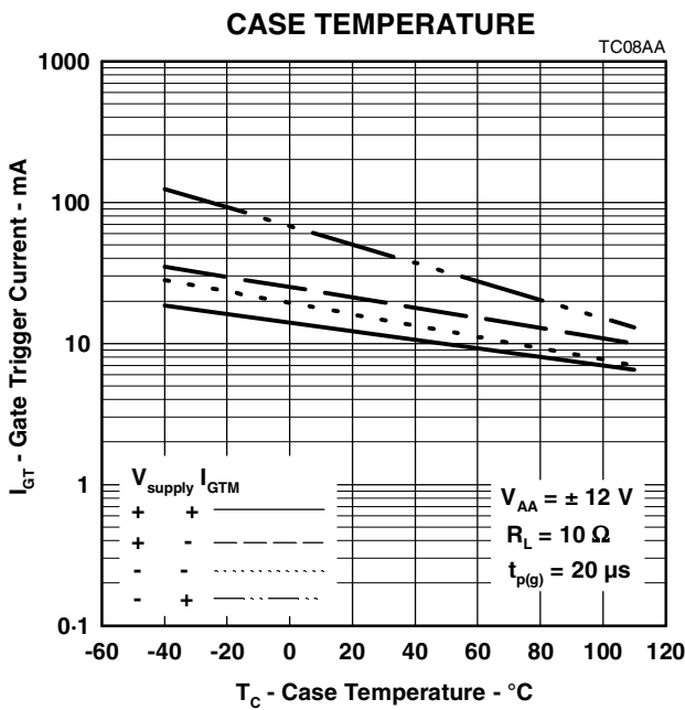
GATE TRIGGER CURRENT VS
