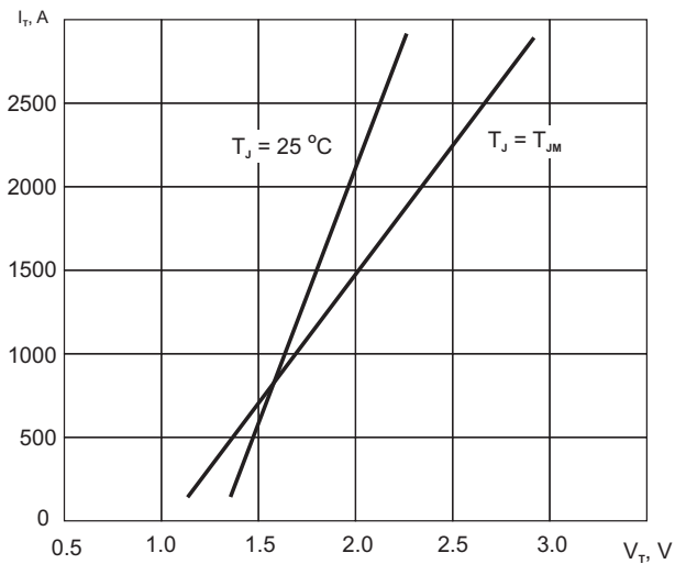
Limiting on-state characteristic I_T = f(V_T)
